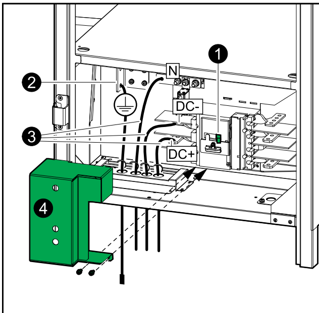
Empty Battery Cabinet – Bottom Cable Entry
